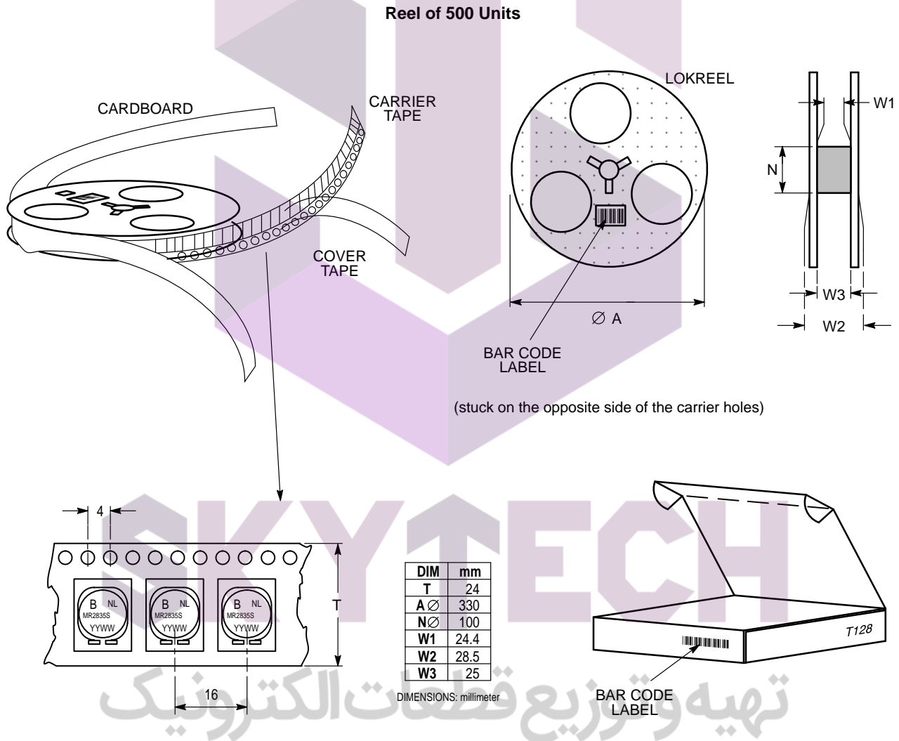
Figure 10. Reel Packing of MR2835S — Top Can
